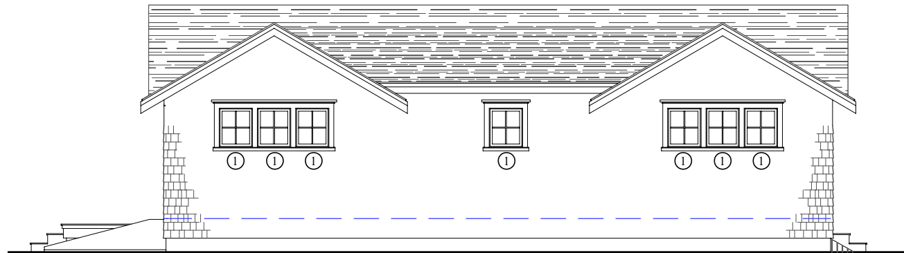
NORTH ELEVATION facing neighbor
