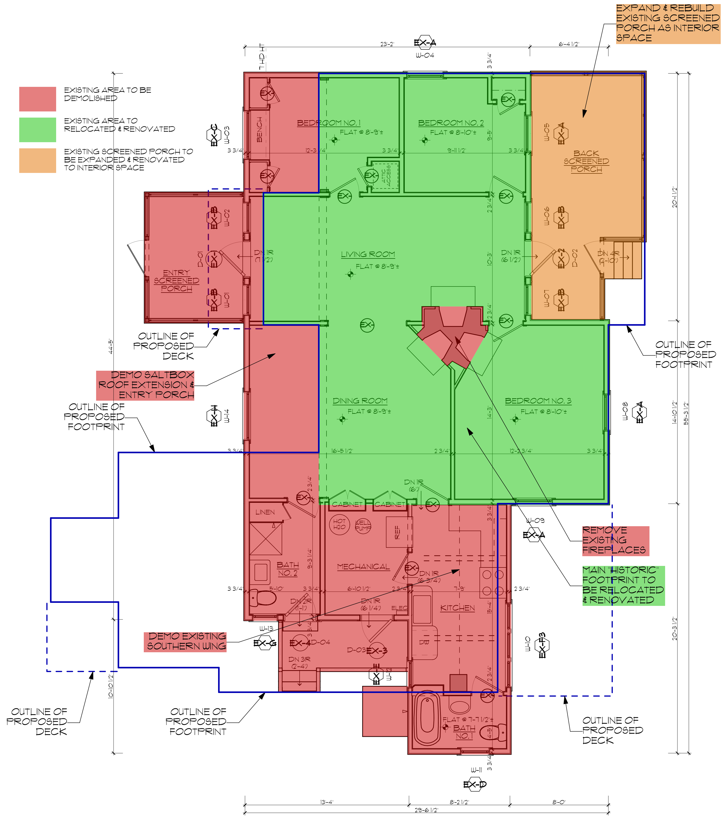
1 DEMO FIRST FLOOR PLAN Scale: 1/4" = 1'-0"
