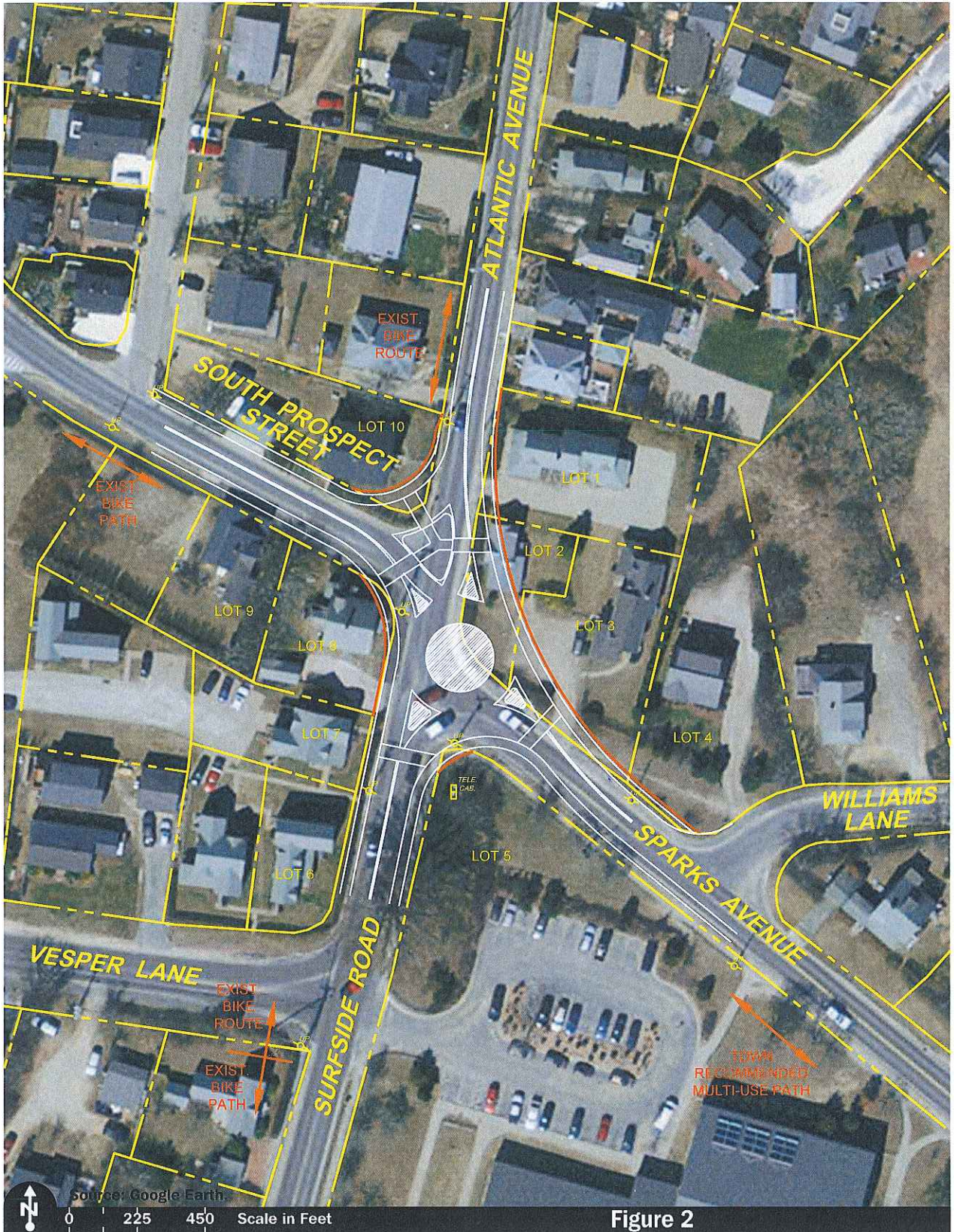
Conceptual Improvement Plan "Four Corner" Intersection
